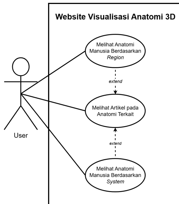
Gambar 3.9: Use case diagram
